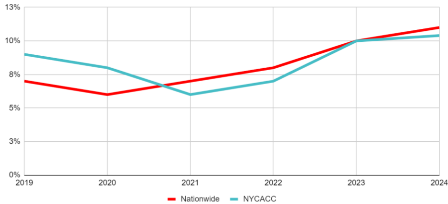
Canine Euthanasia Rates
